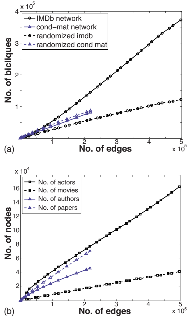
FIG. 5. (Color online) In many sparse real world networks, the number of maximal bicliques grows linearly with the size of the input data base. Panel (a) shows the number of maximal bicliques found for the IMDb [19] and cond-mat [40] networks as a function of size of the networks (measured in number of edges). The solid line labeled by circles shows is the number of bicliques found in the IMDb data and the dashed line labeled by circles is the number of bicliques in the randomized version of the same network; the lines labeled by triangles show the same quantities for the cond-mat network. The network was randomized using a bipartite version of the algorithm suggested in [39]. There are significant differences between the real and randomized data sets in the IMDb data, whereas there is little change for the cond-mat data. These differences are mainly due to the fact that, on average, there are more actors involved in the production of movies than there are authors of scientific papers. A forthcoming paper discusses the subject of biclique motifs in various bipartite networks. Panel (b) shows the growth of the bipartite adjacency matrix as a function of the number of edges included in the analysis; solid line marked by squares is the number of distinct movies and the dashed line marked by squares is the number of actors; the lines labeled by triangles display the number of authors (solid line) and the number of papers (dashed line) for the cond-mat network. The incremental growth of the number of movies in the IMDb network is explained in the main text.
