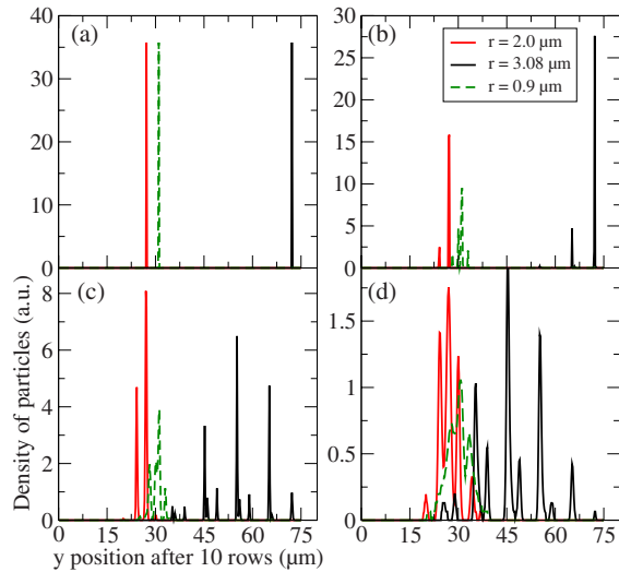
FIG. 5. (Color online) Distributions of three particle sizes: r = 0.90 (dashed line), 2.00 [(red)gray], and 3.08 \mu\text{m} (black) after transport through 10 rows of the N=10 , M=3 array. The total number of particles is the same in each case and each initial distribution (not shown) is a square distribution with a narrow width centered on y=30 \mu\text{m} . (a) No diffusion. (b) With diffusion and v = 1000 \mu\text{m/s} . (c) With diffusion and v = 100 \mu\text{m/s} . (d) With diffusion and v = 10 \mu\text{m/s} . Panel (b) shows a case where mode B_- could be detected experimentally. For the lower speed in panel (c), modes A and B_- cannot be resolved, but the combined distribution is broader than mode A alone. For the even lower speed in panel (d) the distributions of particles in modes A and B_- are each wider than the separation between them and the two modes are completely unresolvable.
