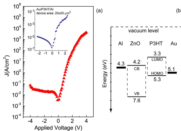
FIG. 3. (Color online) (a) Typical current-voltage characteristics of a 4 \times 4 \mu\text{m}^2 Al/ZnO/P3HT/Au device. In the inset the typical J - V characteristics of an Au/P3HT/Al Schottky junction (Ref. 17) is presented for comparison. (b) Energy band diagram in nonequilibrium conditions of the Al/ZnO/P3HT/Au stack.
