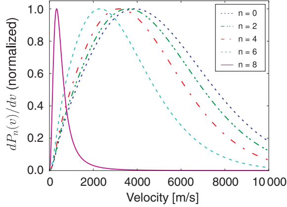
FIG. 1 (color online). Kinetic energy distribution for desorption out of five bound states for the para adsorption site, calculated from Eq. (2). The parameters are given in the text, and \epsilon_i = \epsilon_0 . The probabilities have been normalized to fit the figure, in fact the maximum value of P_n(v) increases by an order of magnitude for each n . The n = 8 state thus has a much larger desorption probability than the rest.
