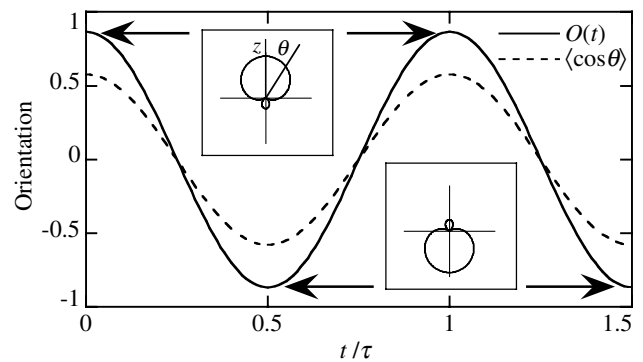
FIG. 1. The principle of field-free orientation—orientation parameters as a function of time. A superposition of the states J' = 0 and (J', M) = (1, 0) (with equal weights) is assumed at t = 0 , in the rigid-rotor approximation. \tau = \pi\hbar/B_e is the fundamental rotational period. The insets show polar plots of the rotational wave function, at the times indicated by the arrows. The complete wave function is obtained by a rotation of the curves about the z axis.
