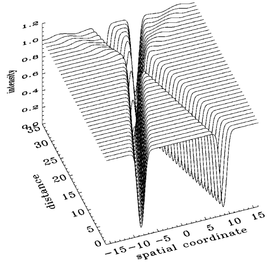
FIG. 9. Propagation and collision of identical dark solitons with \rho_0=10\rho_1=1 in a weakly nonlocal medium with \gamma=0.1 .
