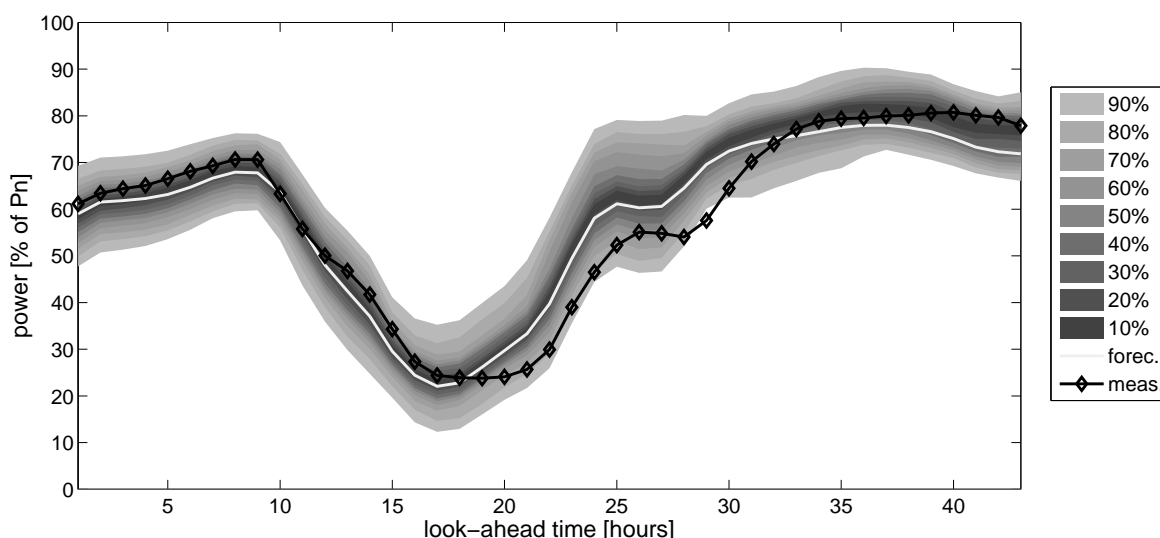
Figure 5. Example of nonparametric density forecasts of wind power generation for the whole Western Denmark (issued on the 8 th January 2007 at noon) in the form of a river of blood fan chart. Density forecasts are represented as a set of central prediction intervals with increasing nominal proportions. Power values are normalized by the total wind capacity P_n for the region. Measurements and point forecasts are also depicted.
