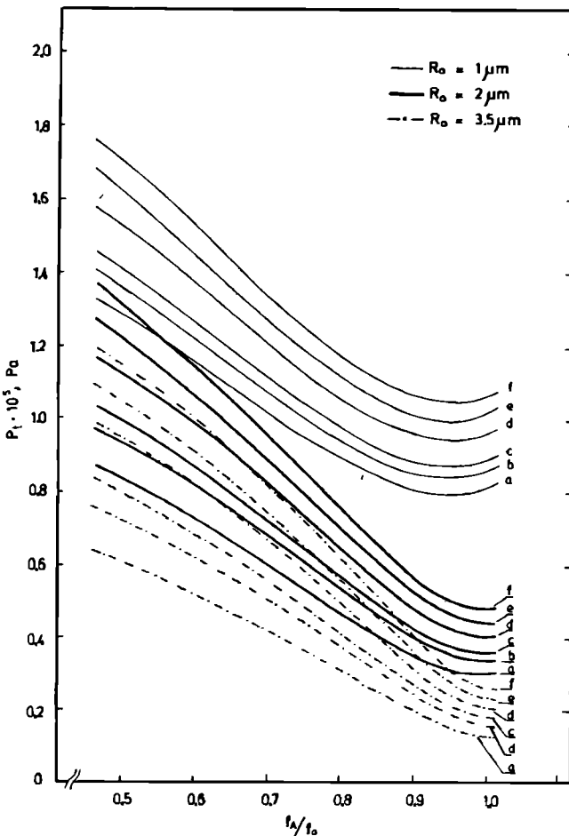
FIG. 3. Peak pressure thresholds P_t for rectified diffusion calculated according to Safar 46 [Eq. (2)] for different relative frequencies f_A/f_0 and concentrations c_1/c_0 : (a) c_1/c_0=1 , (b) c_1/c_0=0.85 , (c) c_1/c_0=0.75 , (d) c_1/c_0=0.5 , (e) c_1/c_0=0.3 , and (f) c_1/c_0=0.1 .
