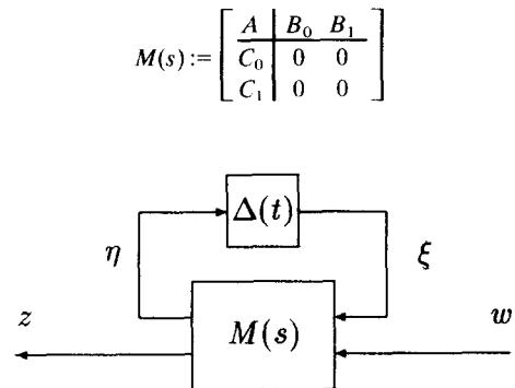
Fig. 1. Uncertainty description.
