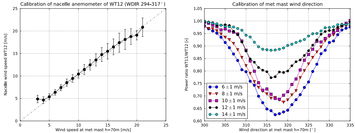
Figure 8. (Left) Correlation between wind speed measured with nacelle-mounted anemometer on WT12 and met mast at hub height. (Right) Power ratio between WT11 and WT12 for wind speed bin intervals; W_{hub} = 6, 8, 10, 12 and 14 \pm 1 \text{ m s}^{-1} as a function of reference wind direction from the met mast.
