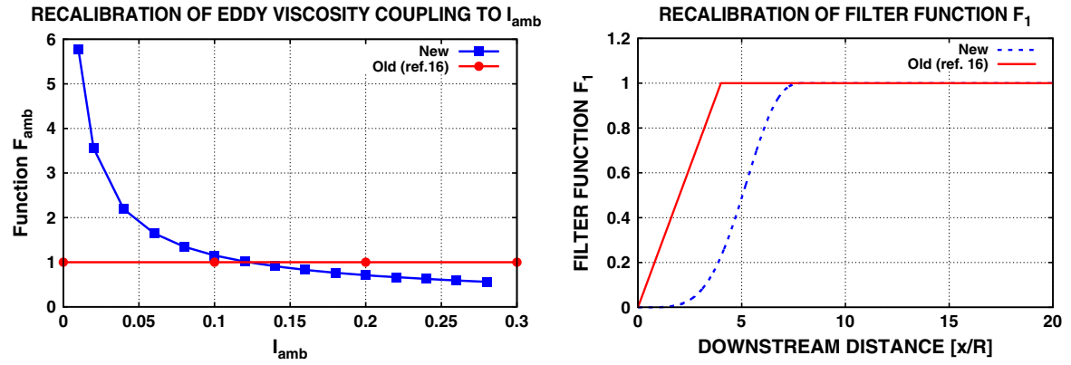
Figure 6. (Left) The new nonlinear coupling function F_{amb} based on a calibration with full-scale measurements of power reduction as function of ambient turbulence. (Right) The modified filter function F_1 based on a calibration with full scale measurements of power reduction as function of ambient turbulence.
