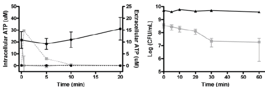
Figure 3.7. ATP leakage from S. aureus after the addition of 1000 µg/mL of chimera 49 (left) and the corresponding change in the number of viable bacterial cells (right). Left: Mean (SEM) intracellular (IC, solid line) and extracellular (EC, punctuated line) ATP concentration for cells treated with chimera 49 (grey) compared to MilliQ-treated control (black). Right: Mean (SEM) number of viable cells after addition of chimera 49 (grey line) compared to MilliQ-treated control (black line). From Paper I.
