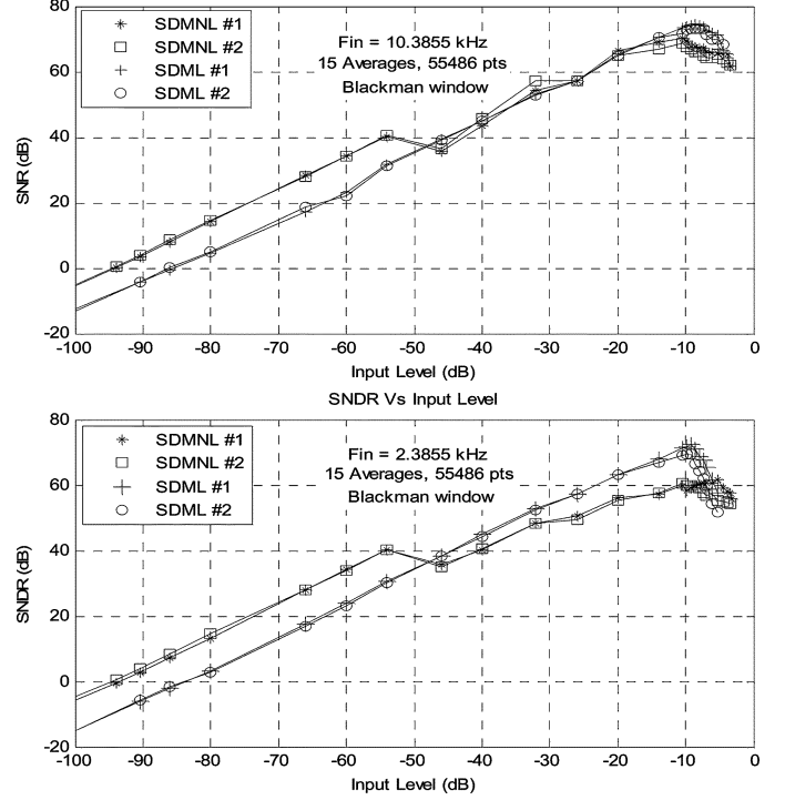
Fig. 9. Measured SNR and SNDR versus input level for two different IC samples of the two \Delta\Sigma Ms (with and without nonlinear DACs).
