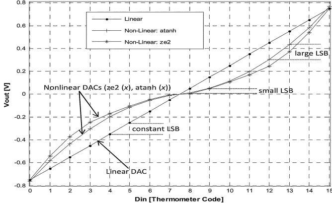
Fig. 2. Conversion steps and DAC conversion characteristics for three different cases (with a linear and two nonlinear 4-bit DAC transfer functions).
