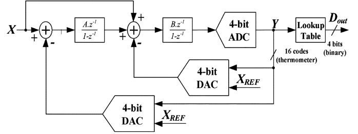
Fig. 1. Architecture of the 2nd-order \Sigma\Delta with feed-forward, a 4-bit quantizer and 4-bit nonlinear DACs ( \Sigma\Delta - 1 ) or 4-bit linear DACs ( \Sigma\Delta - 2 ).
