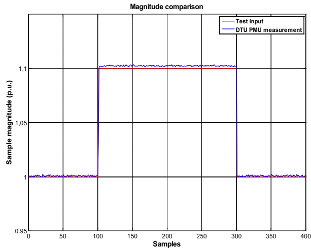
Figure 16 . The response of DTU-PMU in amplitude step test.
