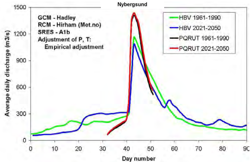
Figure 6.18. Comparison of estimation of the probable maximum flood (PMF) using the PQRUT model with 20-day probable maximum precipitation (PMP) sequence and the HBV model with the PMP sequence and full snow storage and melting routines. The comparison is based on one climate scenario. Results for other scenarios are given in Table 6.2.
