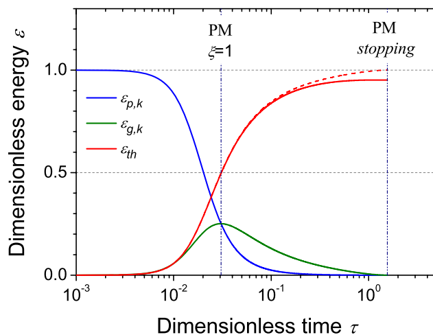
Fig. 2 The components of the dimensionless energy \varepsilon (see (12) and (15)) as a function of the dimensionless time \tau (see (3b)). \varepsilon_{pk} , the kinetic energy of the plume, (see (12b)), \varepsilon_{g,k} , kinetic energy of the background gas (see (12c)), \varepsilon_{th} excess thermal energy of the plume and the background gas (see (15)). The time for \xi = 1 in the PM-model is indicated as well ( v_f/c_g = 31.6 and \gamma_g = 5/3 as in Ref. [9])
