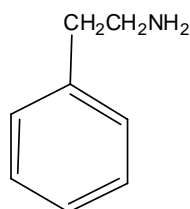
2-Phenylethylamine
