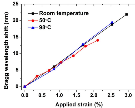
Fig. 6. Large strain response of the 180 \mu\text{m} TOPAS FBG at room temperature, 50°C, and 98°C
