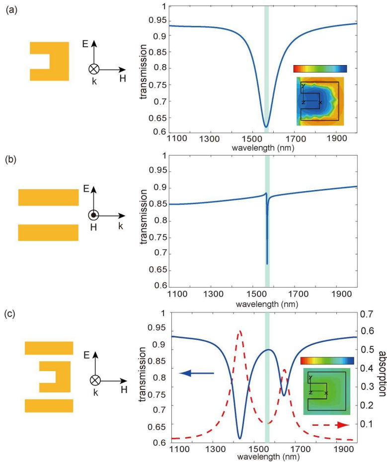
Fig. 1. Schematic of the metamaterial geometry and the incident light polarization. Here L1 = 360\text{nm} , W1 = 95\text{nm} , W2 = L2 = 200\text{nm} , w = 80\text{nm} , d = 100\text{nm} .
