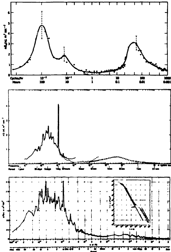
Fig. 6. Three composite spectra of the horizontal wind speed measured from top to bottom at: Brookhaven, U.S.A. (Van der Hoven, 1967); Rissø, Denmark; Munich, Germany (F. Fiedler, 1971). The heights are 100, 5, and 50 m respectively.
