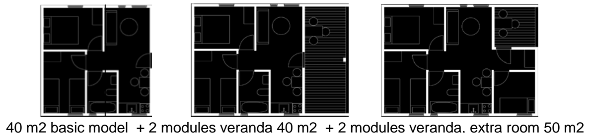
Figure 6: A Type 1 house assembled from prefabricated HPC elements
