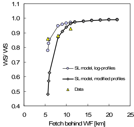
Figure 10 Roughness change model including effect of boundary layer
