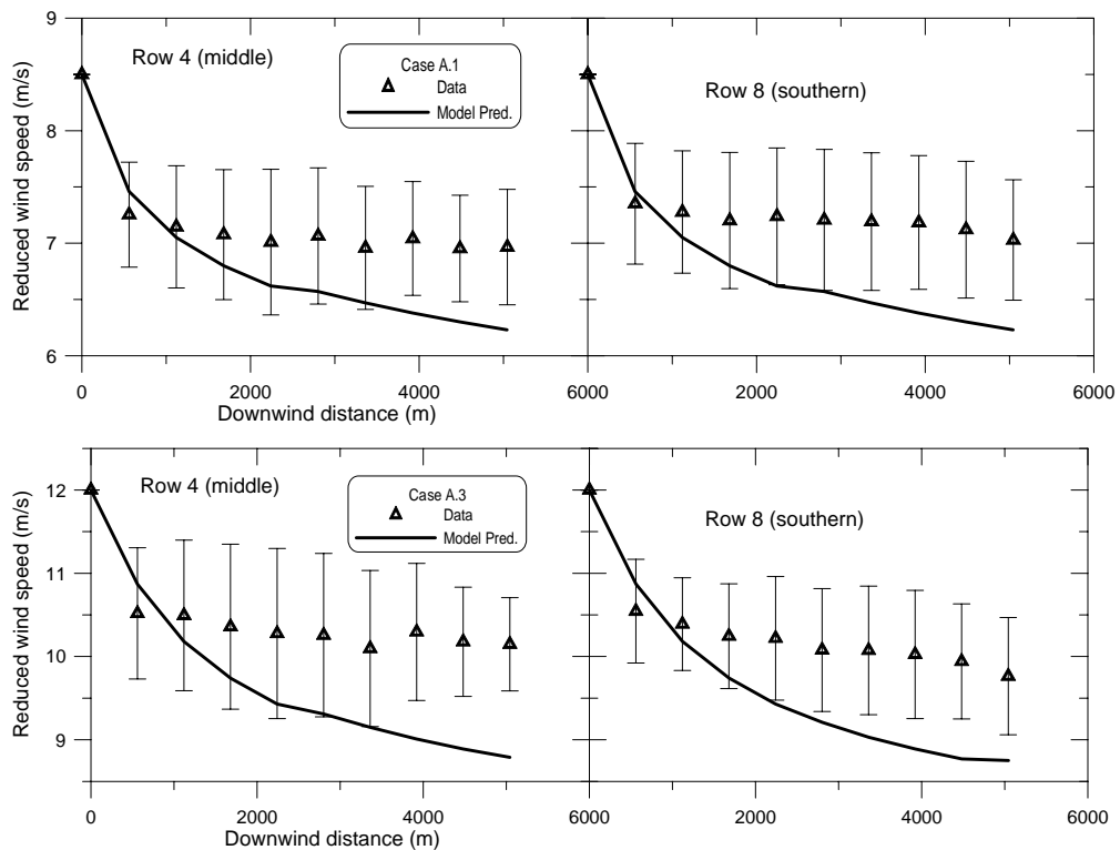
Figure 16. Model predictions at wind direction 270^\circ \pm 3^\circ compared to data. Free wind speed: 8.5 m/s \pm 0.5 m/s (top) and 12.0 m/s \pm 0.5 m/s (bottom).
