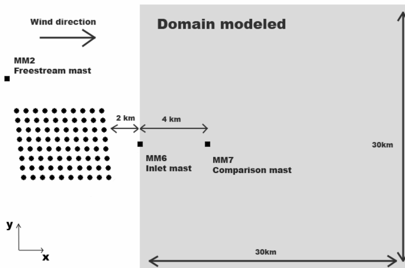
Figure 23. Model Setup.
