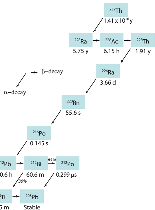
Figure 3-2. The thorium decay series.
