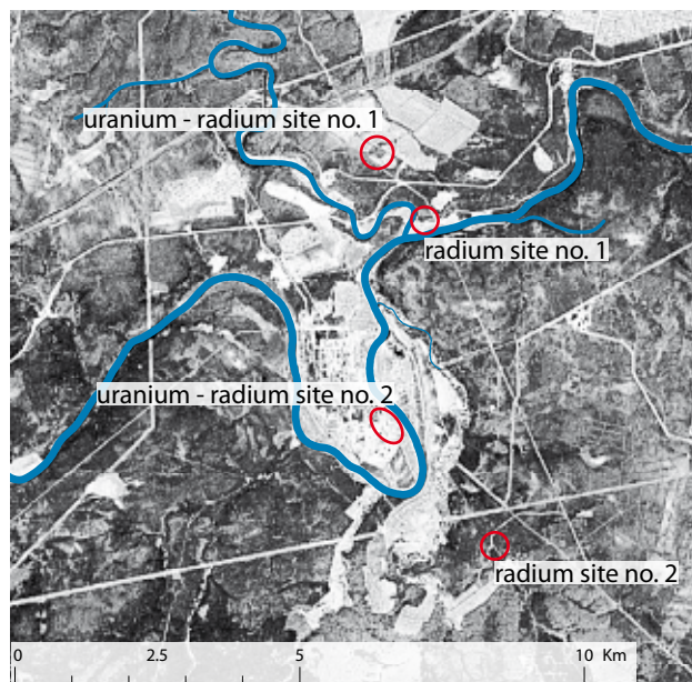
Figure 5-7. Approximate locations of the Vodnyi study sites: Obzhig (U-Ra site 1), Krokhal (Ra site 1), and Otvally (U-Ra site 2).
