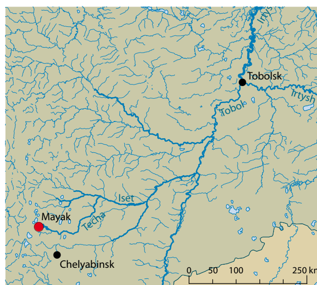
Figure 2.3. The Mayak PA is located at the head of the Techa river, part of the Techa-Iset-Tobol-Irtysch-Ob river system that flows into the Kara Sea.
