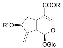
3 R''=R'''=H; gardoside 3a R''=caffeoyl; R'''=1-mannityl; lavaudioside B
