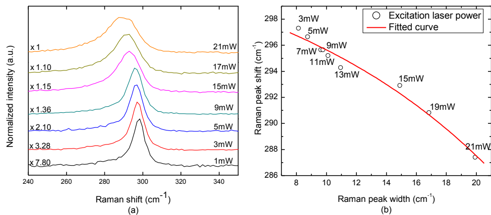
Fig. 4. (a) Raman spectra for sample Ge1_B with varied excitation powers from 1mW to 21mW, (b) Raman peak shift and FWHM with relation to the excitation powers.
