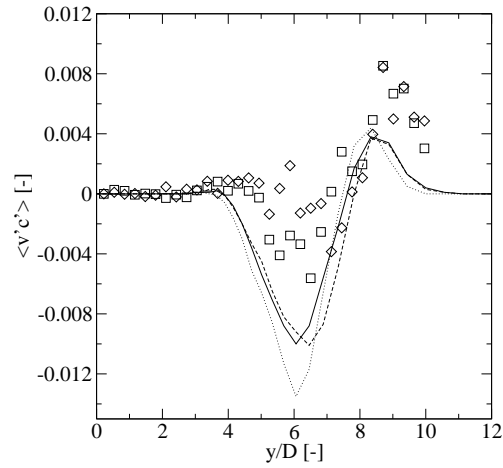
Figure 27: Computed (c) and measured (m) turbulent flux \langle v'c' \rangle on a vertical line in the centerplane at z/D=8 : Round (c) —, square (m) \square , square (c) \cdot\cdot\cdot , diamond (m) \diamond , diamond (c) - - -
