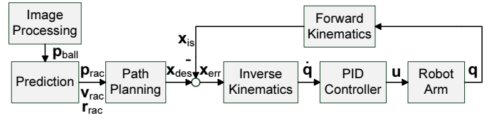
Fig. 5. Control diagram of humanoid 7-DOF robot arm
