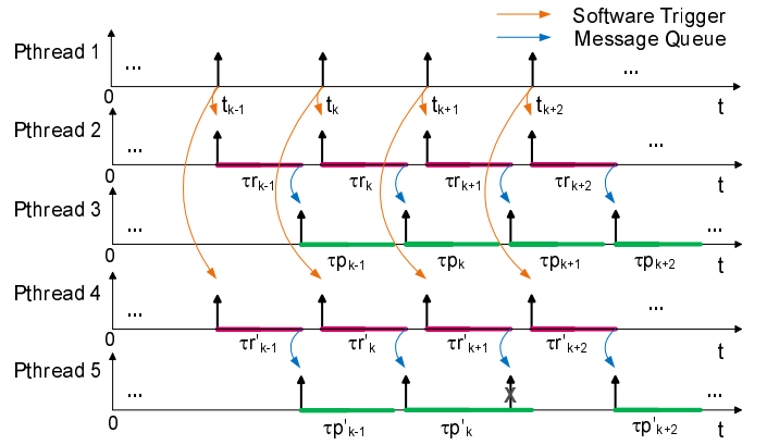
Fig. 3. Parallel processing of vision system
