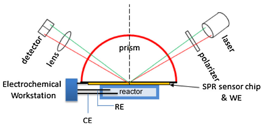
Scheme 1. Scheme of EC-SPR setup.
