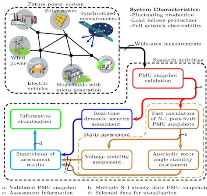
Figure 1: Overview of research activities in the SOSPO project related to real-time security assessment based on synchronphasor measurements.
