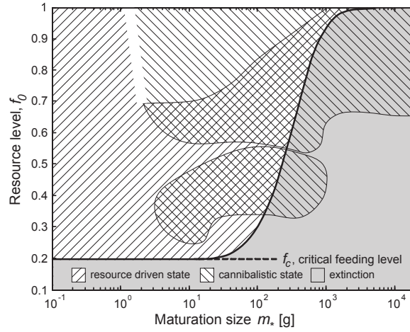
Figure 2: Single-species population states as a function of maturation size and resource level. Invasion from small numbers is possible if the resource level is above the critical level and if the species' maturation size is small enough to allow survival on resources only (white background). Hatching type indicates if the species has a resource-driven or a cannibalistic state (cf. legend). Areas with cross-hatching indicates bistability between the two states, i.e. the species may be in either the resource-driven or the cannibalistic state. The hatched grey area indicates an emergent Allee effect, where only the cannibalistic state exists. The white area in the top left quadrant marks a region where a continuous transition between states occurs.
