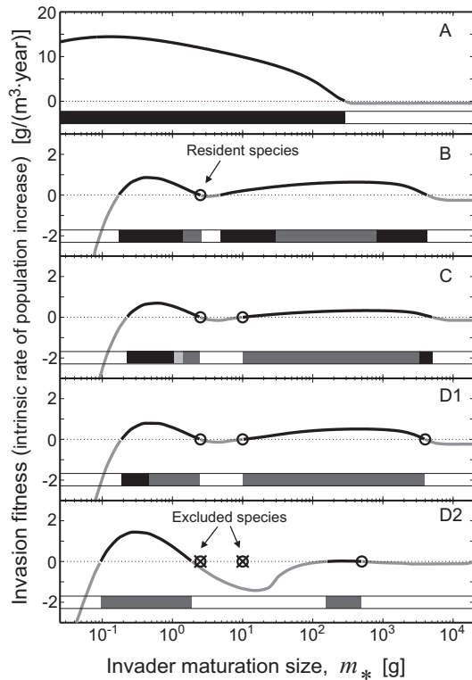
Figure 7: Assembly of a community from a pristine system and up to three coexisting species. Invasion fitness (rate of population increase when the invader is at low density) landscape of pristine system (A), one resident of m_1^* = 2.5 g (B), two residents; m_1^* and m_2^* = 10 g (C), three residents; m_1^* , m_2^* and m_3^* = 4 kg (D1). (D2) illustrates the collapse of the community in (C) due to the introduction of an invader with m^* = 500 g. Invasion fitness of the invader is shown with solid lines, which are black for positive values and grey for negative values. Under each landscape it is denoted whether invasion leads to coexistence (black), exclusion of one of the resident species (dark grey) or exclusion of both one of the resident species and the invader (light grey).
