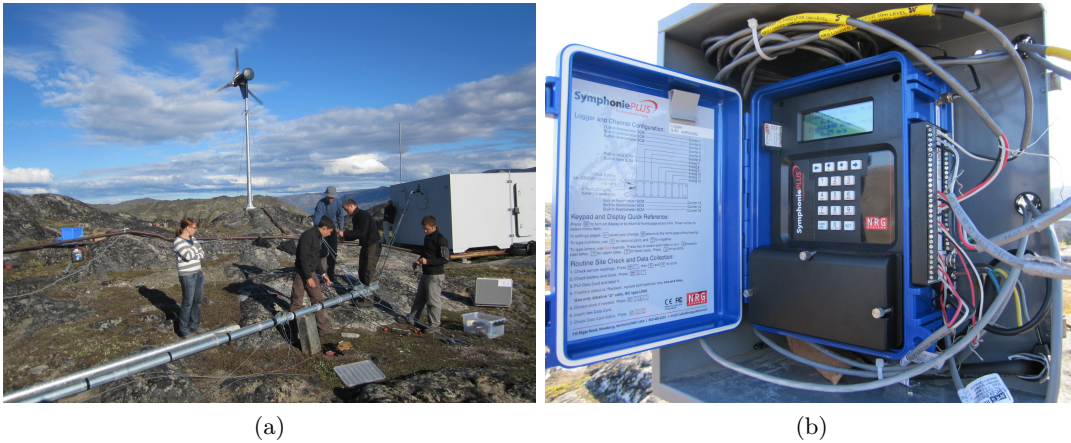
Figure 2.3: Work on the old met. mast at Sarfannguaq. (a) Cabling and anemometers mounting - (b) Configuring the new data-logger with i-Pack
