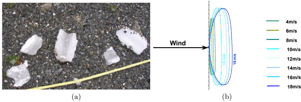
Figure 7.11: Ice throws. (a) Photo of ice fragments [11] - (b) Results of ice throw calculation[19]
