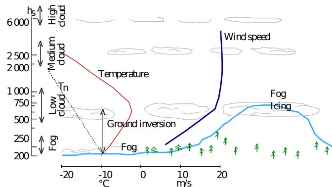
Figure 6.3: Illustration of in-cloud icing, and the difficulty to use meteorological station measurements[56]
