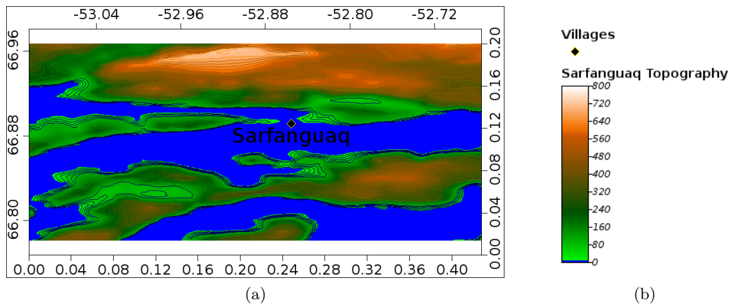
Figure 2.1: Topography of Sarfanguaq in longitude and latitude coordinates. (see Sect. 4.2 for details of the realization of this map with SAGA)
