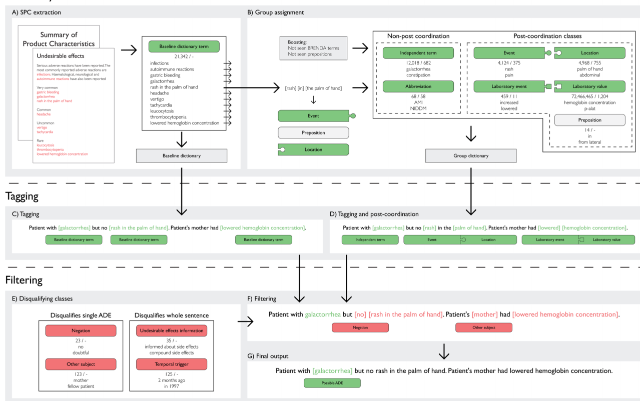
Figure 1 Method flowchart. (A) Adverse event descriptions were extracted from the summaries of product characteristics (SPCs), representing the baseline dictionary. (B) The lexemes in the baseline dictionary were assigned into seven dictionary groups, split in two groups according to whether they are involved in post-coordination or not. The first number below each group indicates the number of concepts and the second number the unique identifiers in the group. (C) Tagging using the baseline dictionary. (D) Tagging using the group dictionary and subsequent post-coordination of tagged lexemes. (E) The four filtering groups split according to whether they disqualify sentence subparts or the whole sentence in the filtering step. The number below each group indicates the number of concepts. (F) Filtering, where any disqualified possible ADE is removed. (G) The final output of the pipeline.
