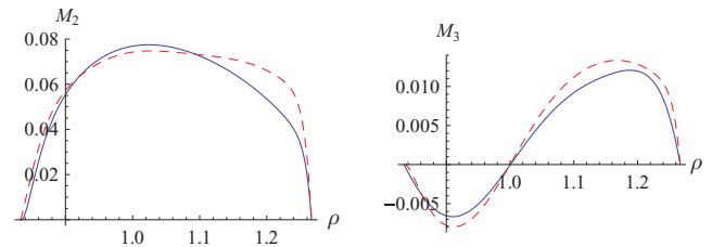
FIG. 9. (Color online) Second and third moments, M_2 and M_3 , of car distribution vs car density \rho in the nonmodulated case. Solid curves obtained from numerical simulations, dashed curves obtained from Eqs. (61) and (62), i.e., interacting mode approach. Parameters: L = 30 , \tau = 0.525 .
