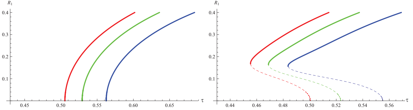
FIG. 7. (Color online) The amplitude of the linearly unstable mode R_1 vs the time relaxation \tau for two values of car density: \rho = 1 (left panel) and \rho = 0.9 (right panel). The dashed curves correspond to unstable branches. From left to right the curves are plotted for safety distance modulation amplitude f = 0 , f = 0.3 , and f = 0.45 , respectively. Other parameters are M = 30 , h = 1 , \Omega = 5 .
