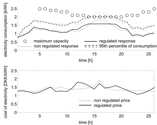
Fig. 11. DEVI group consumption response to CC optimized price signals, when the level of confidence is 1 - \rho = 95\% .
