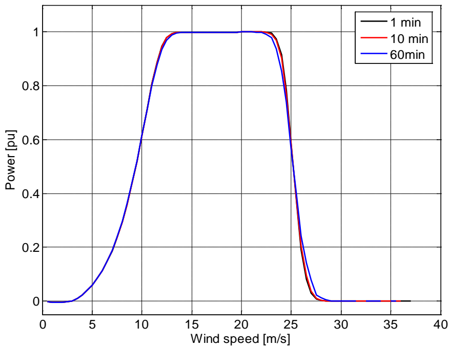
Figure 12 Aggregated wind farm power curve
