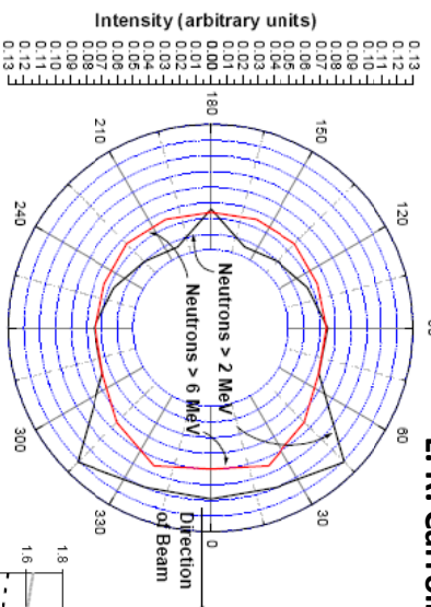
Angular Distribution of Neutrons from O-18(p,n)F-18 at Ep=10.4 MeV
