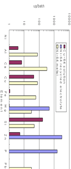
Fig. Metallic impurities in the final 64 Cu solution and 64 Ni electrolyte measured by ICP-MS.
