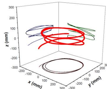
Fig 7: First PEPT run
