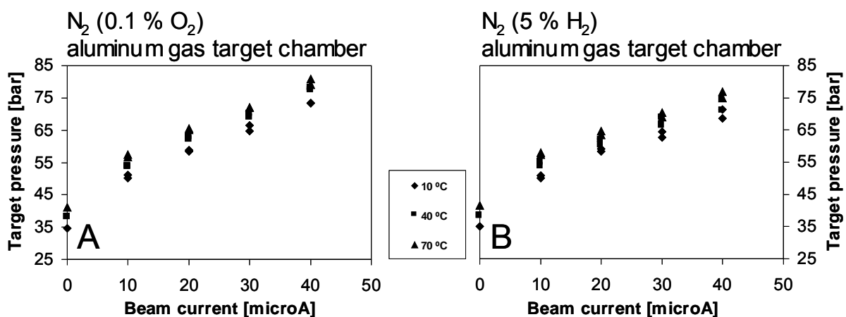
Figure 1. Pressure versus irradiation current at different target body temperatures
