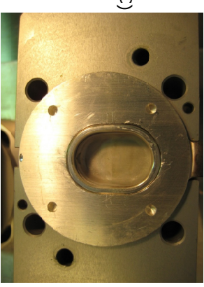
Target cavity of Risø's present target(s) seen from the front. Lateral extent of cavity is larger than new design, but not as deep
