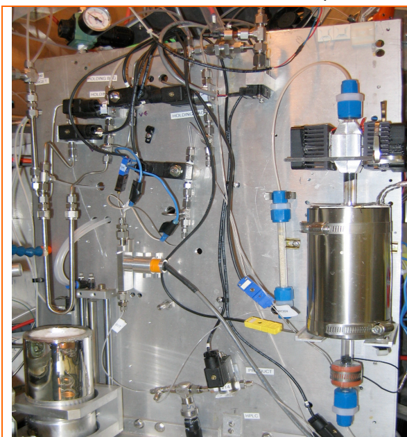
Photograph of New TRIUMF [ 11 C]methyl iodide module. Note the vertically mounted quartz tube in the oven, band heater for iodine vaporization below and Peltier cooling unit for iodine trapping above.
