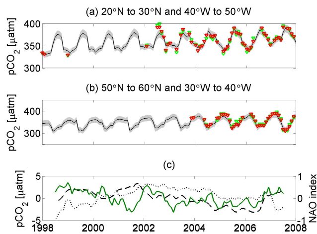
Fig. 13. (a) Temporal evolution of the p\text{CO}_2 (in \mu\text{atm} ) in the subtropical ( 20\text{--}30^\circ \text{ N} , 40\text{--}50^\circ \text{ W} ) and (b) in the subpolar box ( 50\text{--}60^\circ \text{ N} , 30\text{--}40^\circ \text{ W} ). The black line shows the spatial average p\text{CO}_2 within each 10^\circ \times 10^\circ box. Red triangles illustrate the average sea surface measured p\text{CO}_2 within each box where observations are available and the green triangles represent the average of the neural network p\text{CO}_2 of those 1^\circ \times 1^\circ pixels which have co-located p\text{CO}_2 observations in SOCAT v1.5. (c) p\text{CO}_2 anomalies (left axis in \mu\text{atm} – detrended and smoothed using a 12 month running average filter) compared to the NAO index (right axis – smoothed using a 12 month running average filter). The dashed line shows the anomaly for the subtropical box, the dotted line for the subpolar box and the green line illustrates the NAO index.
