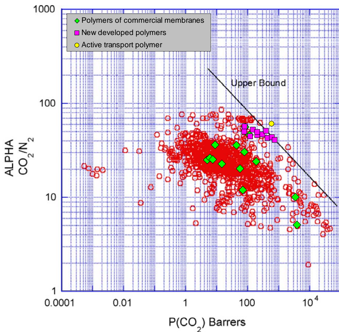
Figure 1. Robeson (2008) plot of \text{CO}_2/\text{N}_2 selectivity vs \text{CO}_2 permeability coefficients with polymers of commercial membranes marked green. New polymeric materials developed in frames of MEMBRAIN project are shown in pink and yellow.
