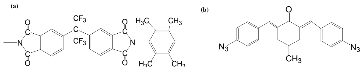
Figure 1. Chemical structures of (a) 6FDA-TMPDA and (b) 2,6-Bis(4-azidobenzylidene)-4-methylcyclohexanone
