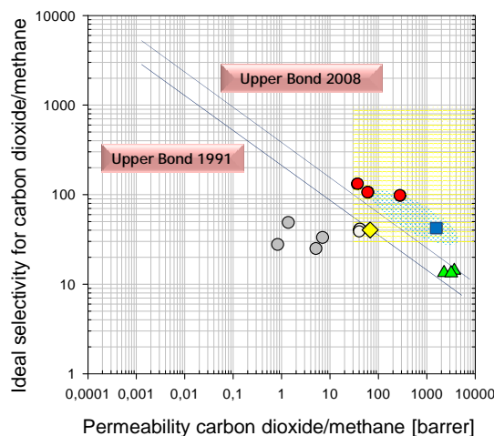
Fig. 1 Upper bond diagram for CO 2 /CH 4 separation, commercial polymers, (○), polymeric materials after thermal rearrangements (■) and green area, PIMs (▲) polymer blends crosslinked and carbonized (●), mixed matrix membranes (◆), area postulated with crosslinked mixed matrix membranes (yellow area)
