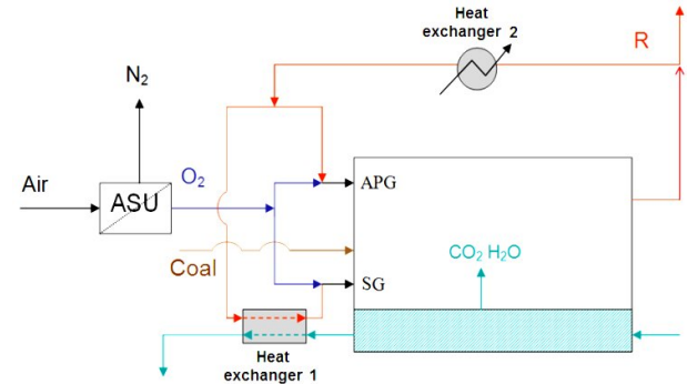
Figure 1. Oxy-fuel process scheme
