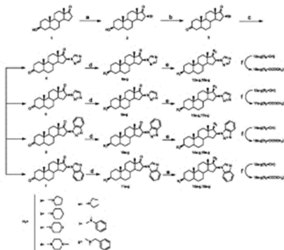
Figure 1. Preparation of target compounds(16a-g,17a-g,18a-g,19a-g). Reagents and Conditions: (a) CuBr 2 , MeOH/d, 65°C, 12h; (b) Jones Reagent, acetone, Isohex; (c) appropriate acids, K 2 CO 3 , CH 3 CN, 65-80°C; (d) appropriate amine, NaBH 4 /CN, MeOH/d, 48°C, 24h; (e) NaBH 4 , MeOH/d, Isohex, 4h; (f) Acetic Anhydride, 4-Dimethylaminopyridine, CH 2 Cl 2 , 48°C.
