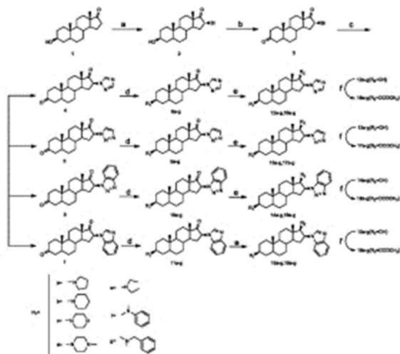
Figure 1. Preparation of target compounds(16a-g,17a-g,18a-g,19a-g). Reagents and Conditions: (a) \text{CuBr}_2 , Methanol, 55^\circ\text{C} , 12h; (b) Jones Reagent, acetone, toluene; (c) appropriate aryls, \text{K}_2\text{CO}_3 , \text{CH}_2\text{CN} , 65-80^\circ\text{C} ; (d) appropriate aryls, \text{NaBH}_4/\text{CN} , Methanol, 40^\circ\text{C} , 24h; (e) \text{NaBH}_4 , Methanol, toluene, 4h; (f) Acetic Anhydride, 4-Dimethylaminopyridine, \text{CH}_2\text{Cl}_2 , 40^\circ\text{C} .
