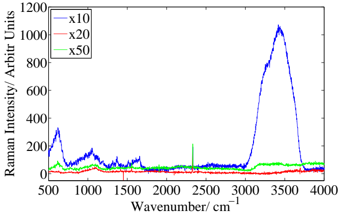
Figure 2.11: Spectra of the colloids taken with the clean lenses, x10, x20 and x50. It can be seen that lens x10 has a lot more feature because of its larger focus area. The peak at 2336\text{ cm}^{-1} is due to \text{N}_2 in the air, while the peak at 1558\text{ cm}^{-1} is due to \text{O}_2 . Mode 1, micro, alu plate, 250mW
