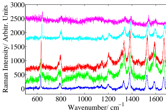
Figure 2.8: C12/ABT solution: 10^{-6} M with colloids [C12/ABT : colloids]=4:6. Vary NaCl from 1\mu\text{L} to 5\mu\text{L} , bottom-up. Displayed with an offset. Model, micro, alu plates, 250mW, x20 lens.
