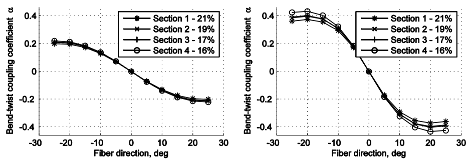
Figure 21 Variation of the normalized bend-twist coupling coefficient of wind turbine blade sections. (a) GFRP. (b) CFRP.
