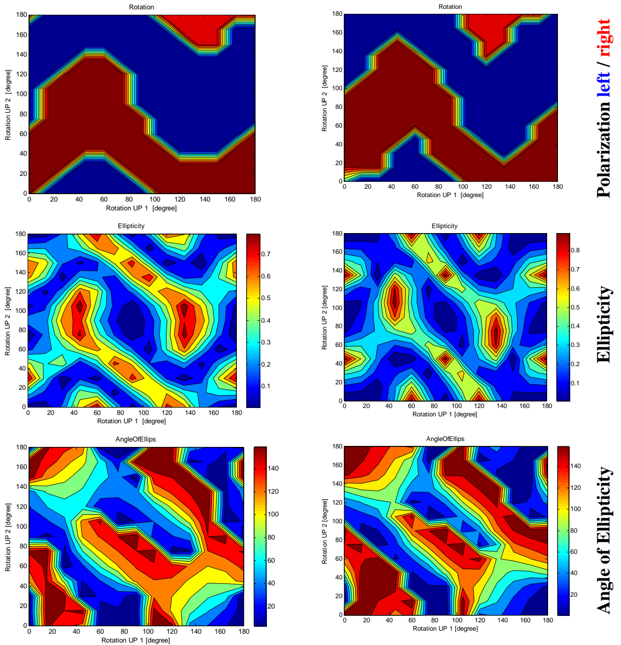
Measurement Calculation Figure 17. Comparison between measurement and calculation of light characteristic of the 110 GHz gyrotron at TEXTOR. Resolution: 15° steps.
