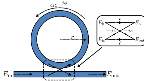
Figure 2.1: Model of basic configuration of MRR: a single ring resonator with one straight waveguide.
