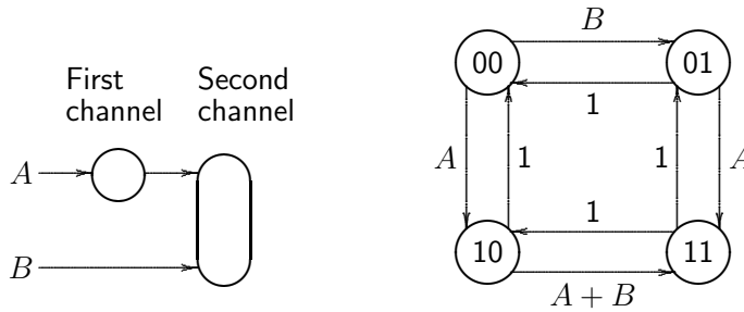
Fig. 2. Two channels, static reservation: the model and the state transition diagram.
