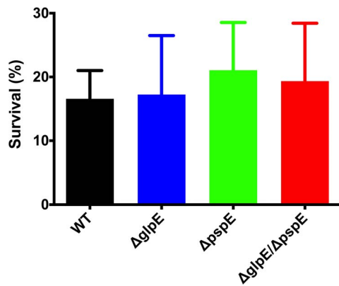
Figure 3. Survival of wild type 4/74 and \Delta pspE , \Delta glpE and \Delta pspE/glpE strains in the presence of peroxynitrite treatment.
