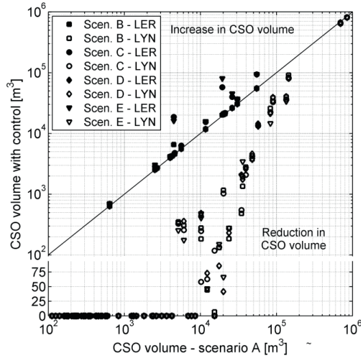
Fig. 5. Comparison between CSO event volumes for the baseline (scenario A – on the X-axis) and for different control scenarios at Lersoeledning and Lynetten (Note the different scale on the Y-axis).
