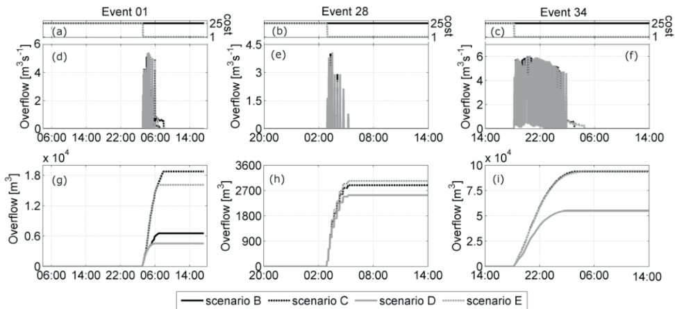
Fig. 6. Simulated CSO costs (a,b,c), overflows (d,e,f), and cumulated CSO volumes (g,h,i) at Lersoeledning for the three sample events.
