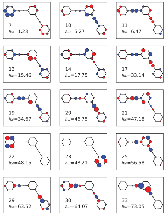
FIG. 6. Out-of-plane modes for meta-OPE3 within the transport energy window. For each mode we indicate the mode index and the eigen-energy (in units of meV).
