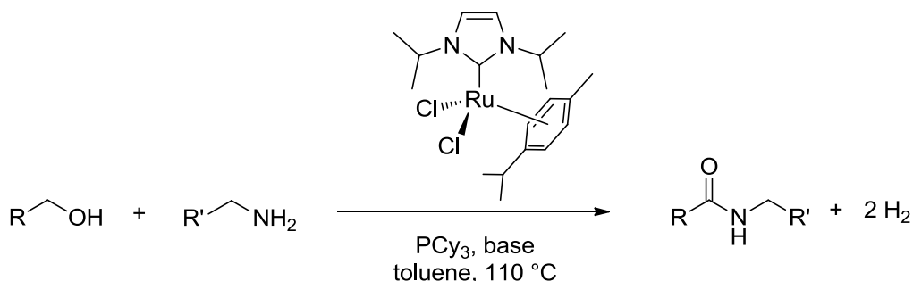
Scheme 1. Amide synthesis.
