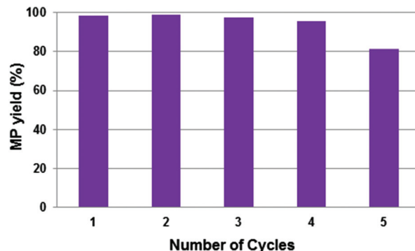
Fig. 4 Recycling experiments using the BAIL [SBMI][ p -TsO] (3) as reaction media and an acid promoter in the methoxycarbonylation of ethylene (reaction conditions: 0.05 mmol Pd(OAc) 2 (0.3 mol% Pd), DTBPMB : Pd mol ratio = 5 : 1, 6 mL of a 32 wt% solution of BAIL in methanol, P(CO : C 2 H 4 : Ar = 2 : 2 : 1) = 22 bars, T = 80 °C, t = 20 min).
