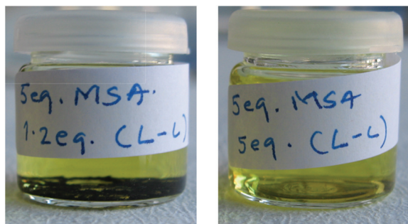
Fig. 3 Reaction mixtures after Pd–DTBPMB catalyzed ethylene methoxycarbonylation with MeSO 3 H as an acid promoter and DTBPMB : Pd ratio = 1.2 : 1 (left) and DTBPMB : Pd ratio = 5 : 1 (right).
