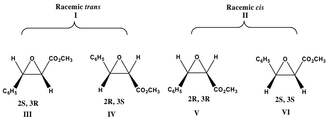
Figure 1: Structures and absolute configurations of optically active trans- and cis-methyl epoxypropenoate (3-phenyl-2,3-epoxypropenoate) and the urinary metabolites isolated from rats. (From (Rietveld et al., 1988))
